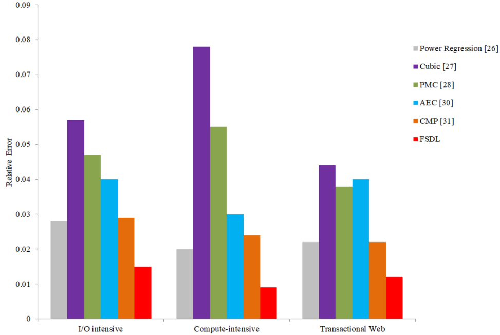
Fig. 4 Comparison of relative errors of different models
