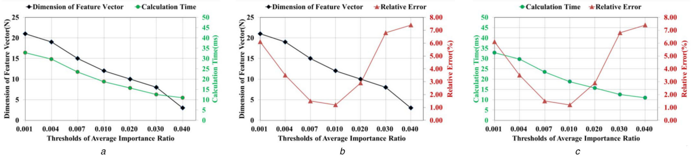
Fig. 3 Experimental comparison of different thresholds
