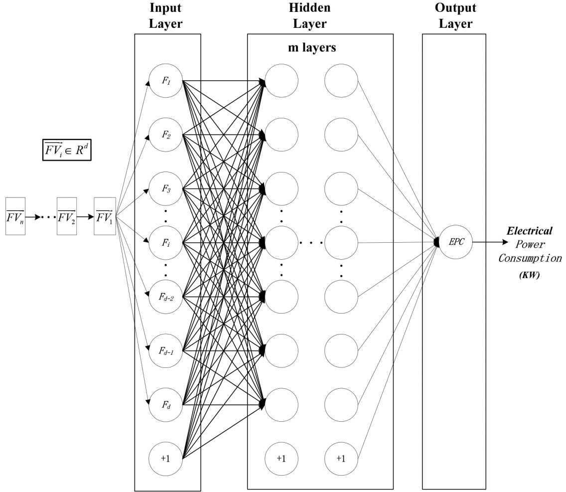
Fig. 2 Deep neural network architecture
